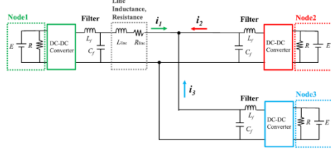
Fig. 4. Circuit configuration of distribution network with three nodes and three converters for validation of power flow control.
