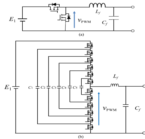
Fig. 2. Circuit configurations of power flow controllers. (a) Two-level topology. (b) Multi-level topology (seven-level case).
